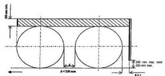
(a) Multiple axles where the distance between the axles is less than 250 mm.
