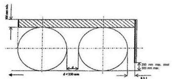
(a) Multiple axes where the distance between the tyres is less than 250 mm.
