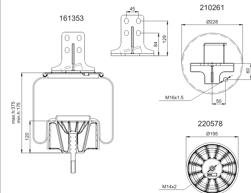
(Composite Piston)
