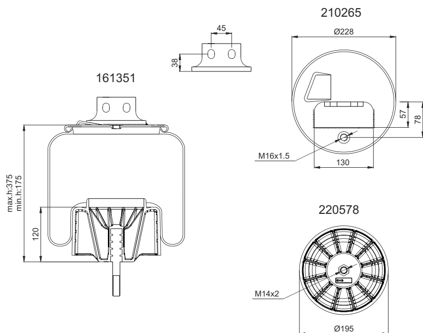
(Composite Piston)
