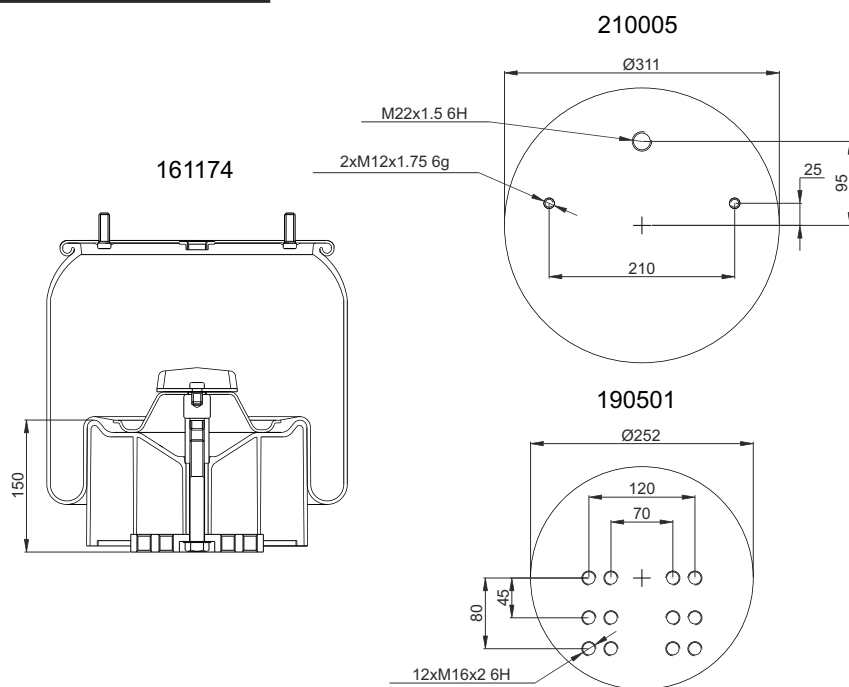
(Composite Piston)
