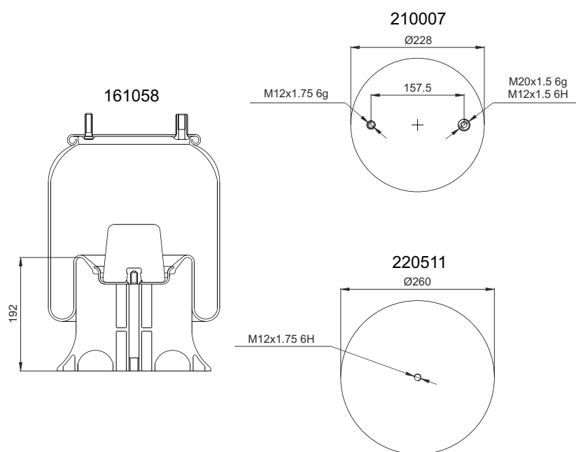
(Composite Piston)
