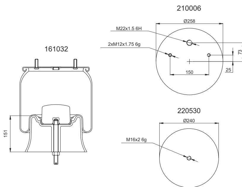
(Composite Piston)
