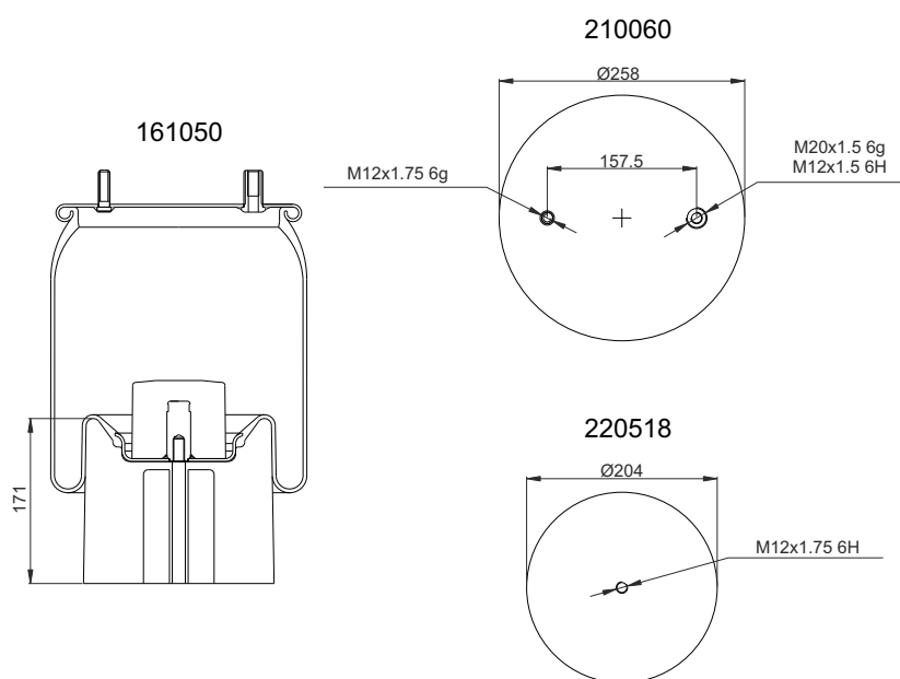
(Composite Piston)
