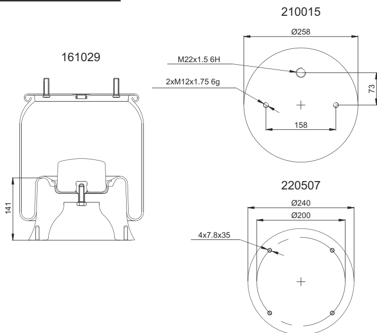
(Composite Piston)
