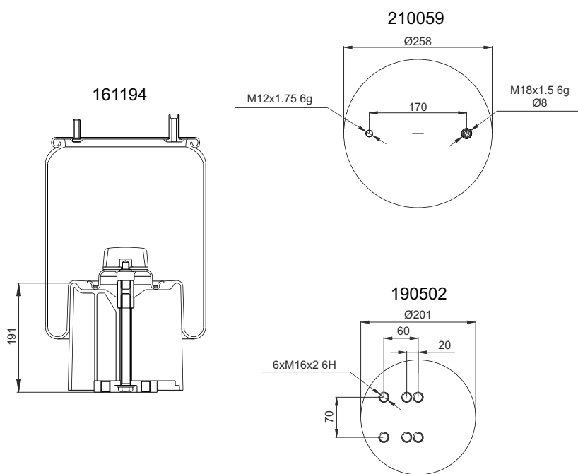
(Composite Piston)
