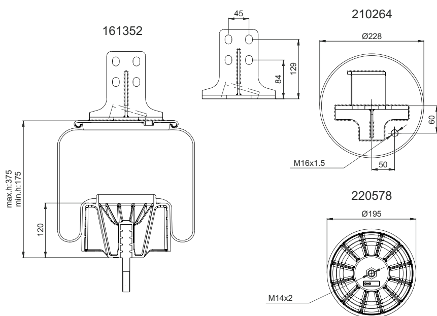
(Composite Piston)
