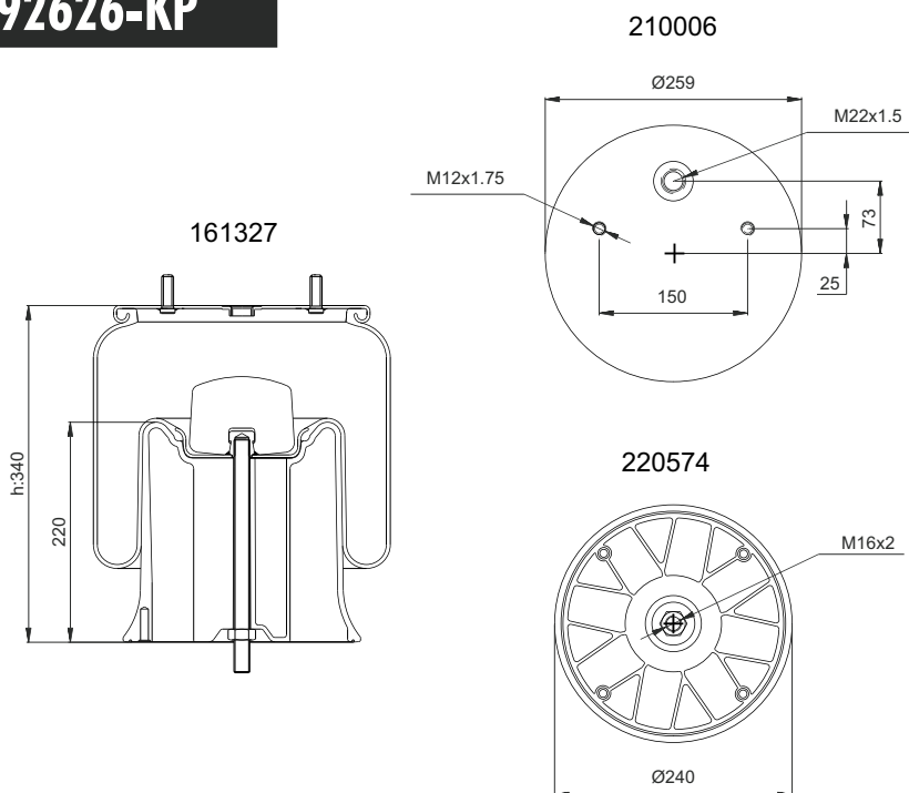
(Composite Piston)
